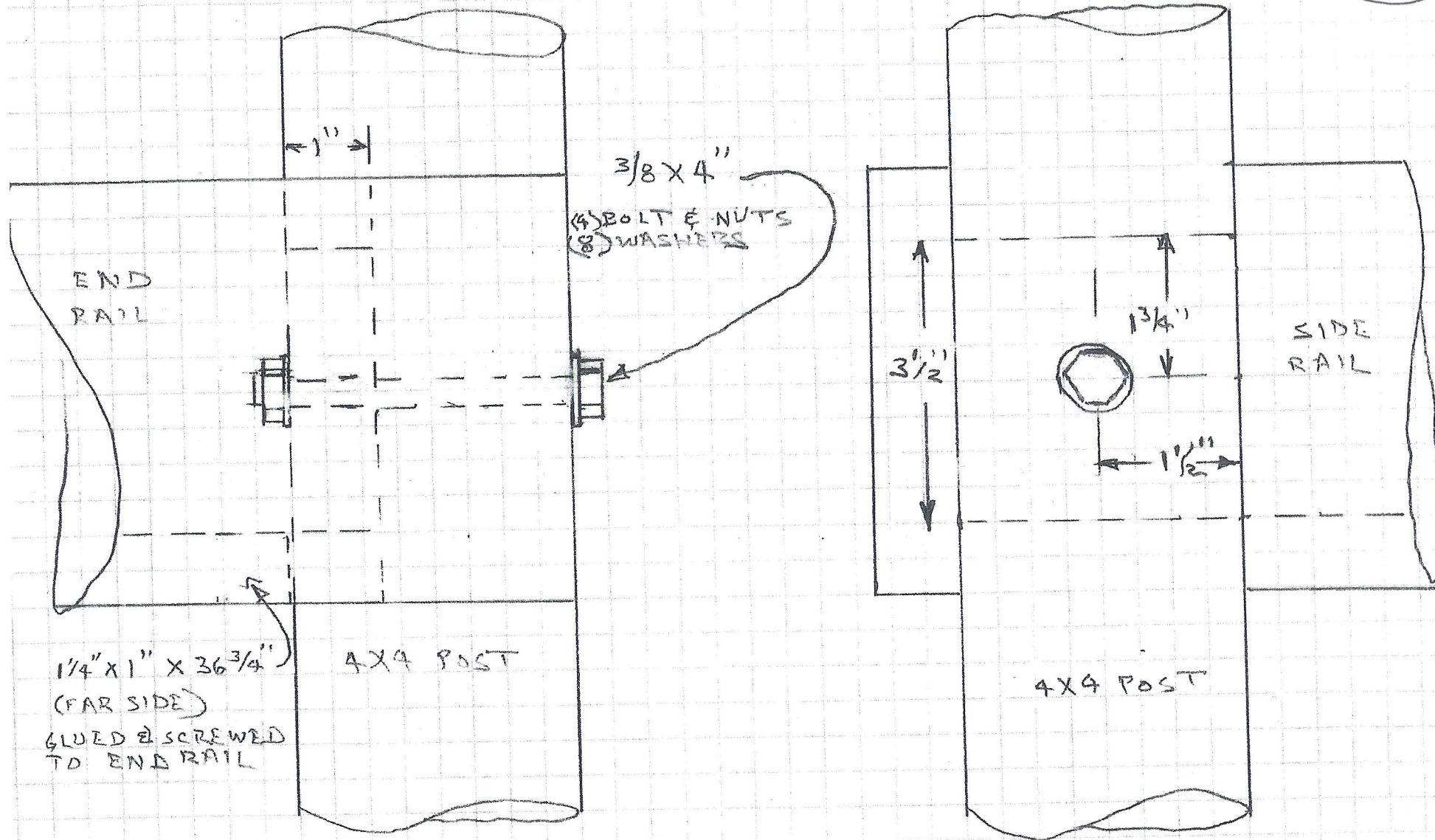
POST TO SIDE RAIL DETAIL A
